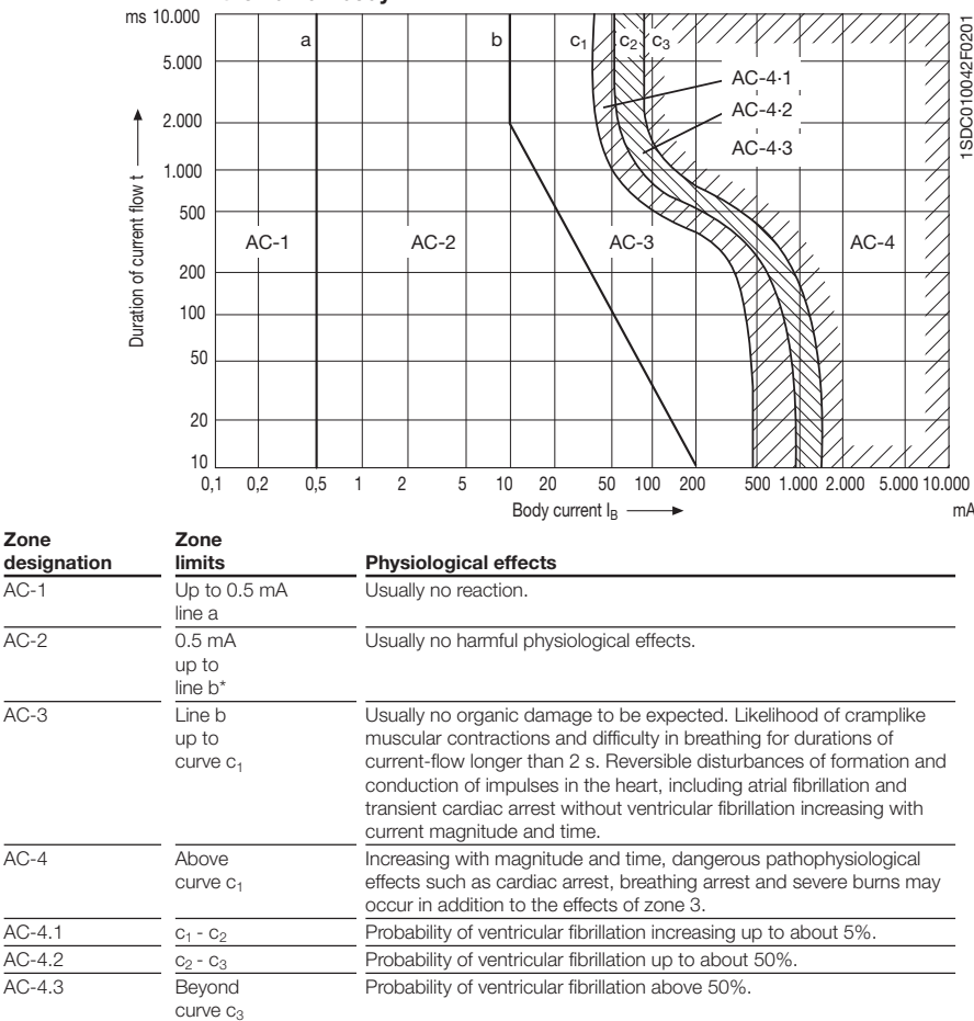
Figure 1: Time-current zones of the effects of alternating current on the human body
