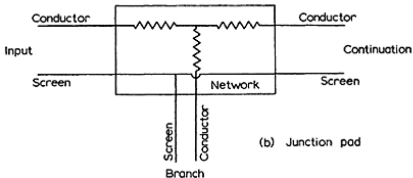
Figure 13.13 Junction box
