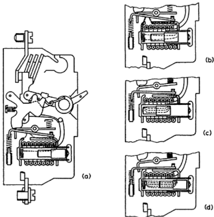
Figure 9.7 Circuit breaker
