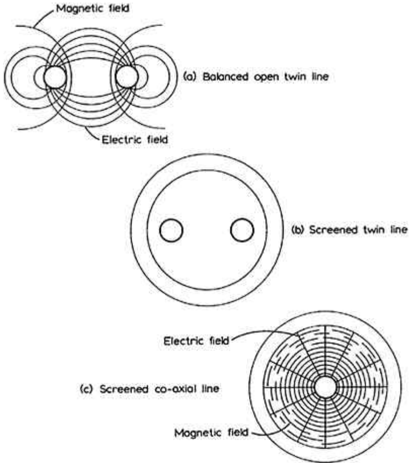
Figure 13.14 TV cables
