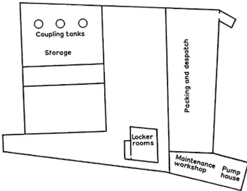
Figure 18.5 Factory first-floor equipment layout
