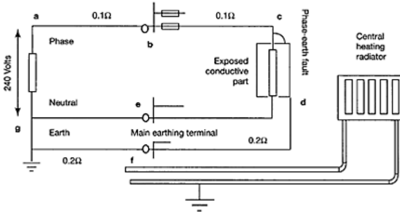
Figure 9.12a Fault currents
