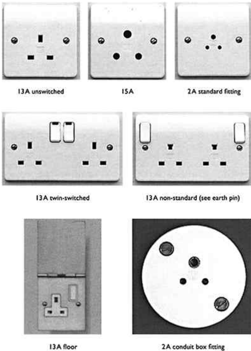
Figure 1.5 Socket outlets (Courtesy of M.K. Electric Ltd)
