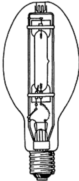
Figure 7.6 MBF lamp
