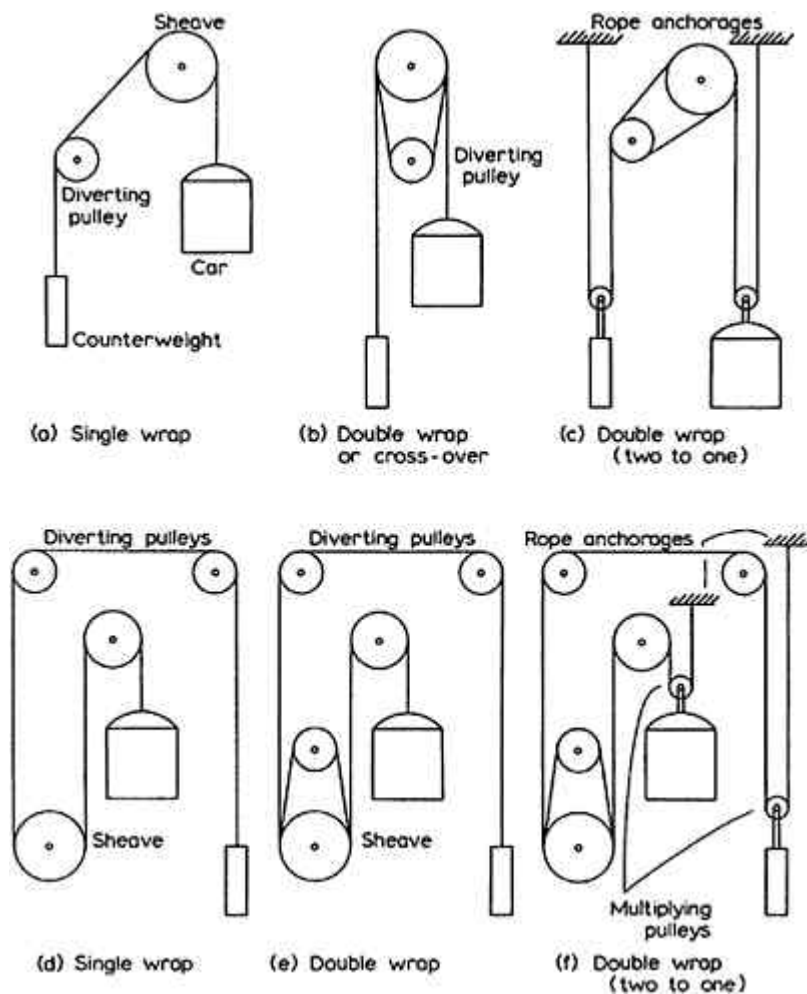
Figure 16.3 Roping systems
