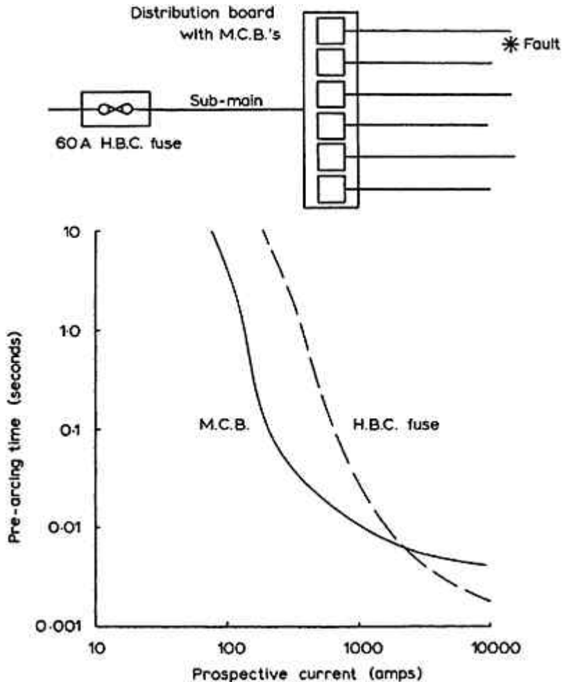
Figure 9.13 Discrimination
