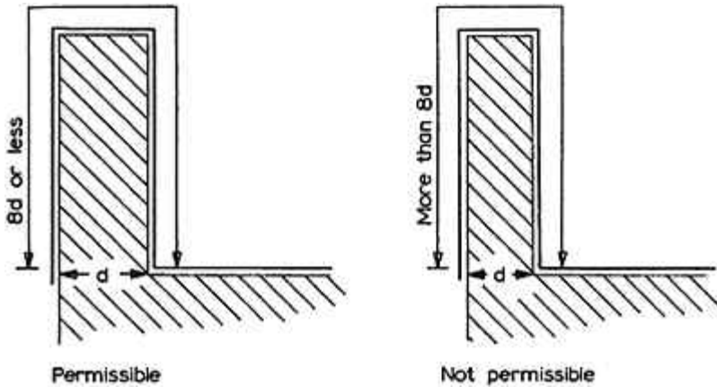
Figure 14.7 Re-entrant loops
