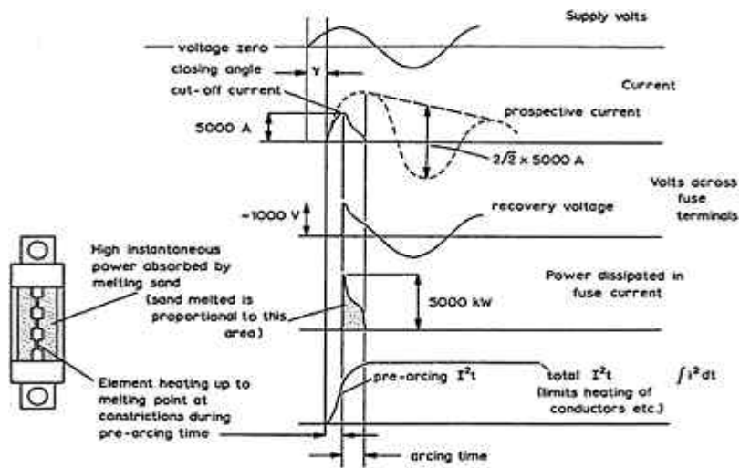
Figure 9.6 Oscillograms of fuse operation
