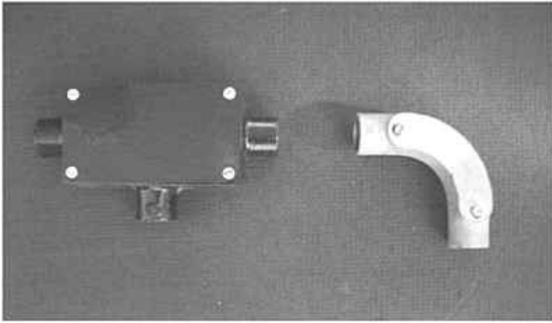
Figure 3.3 Conduit inspection fittings
