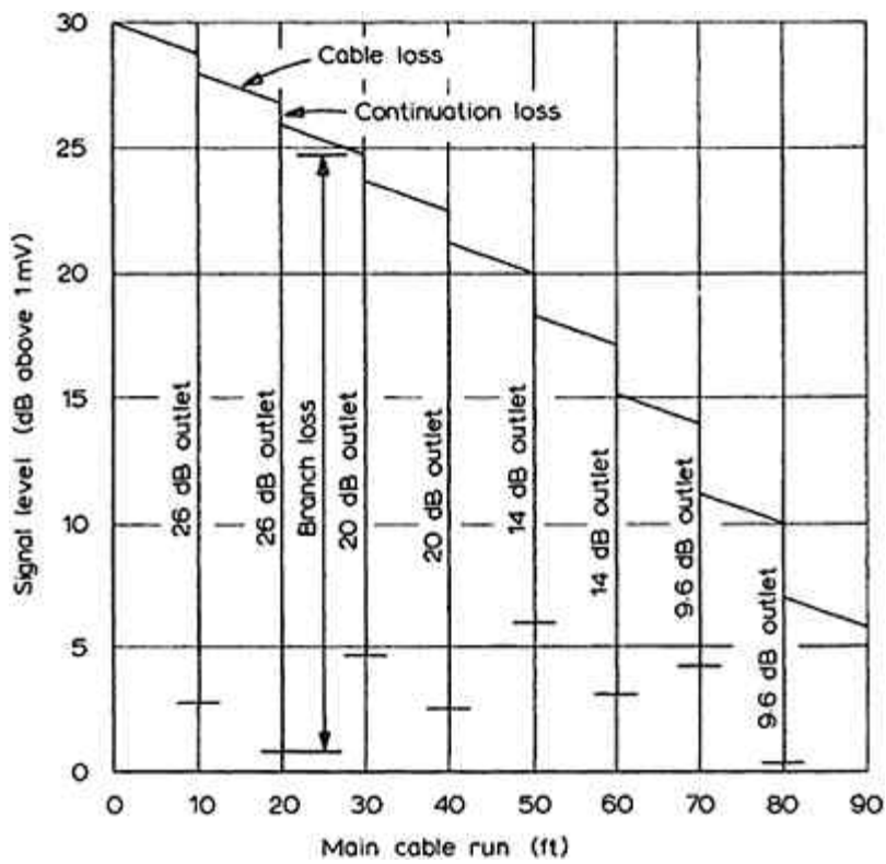
Figure 13.16 Attenuation graph
