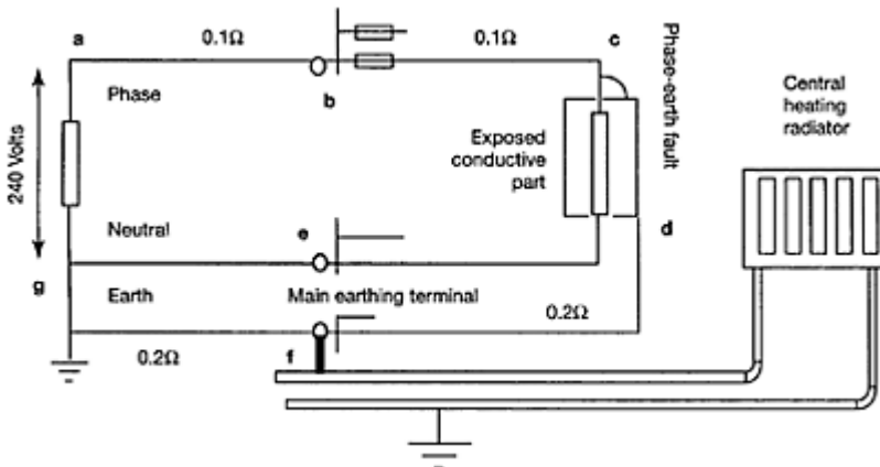
Figure 9.12b Fault currents
