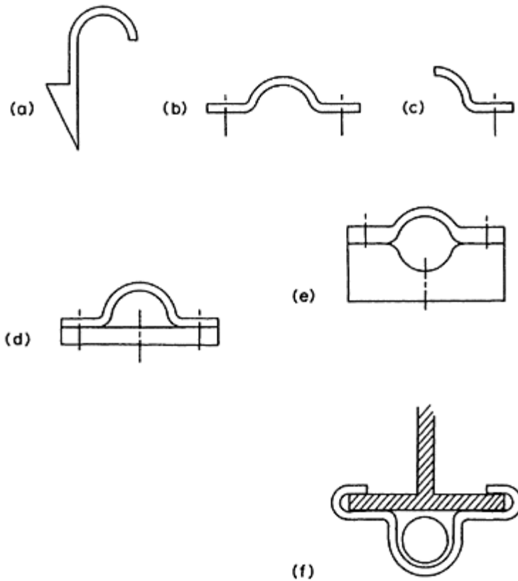
Figure 3.10 Conduit fixings
