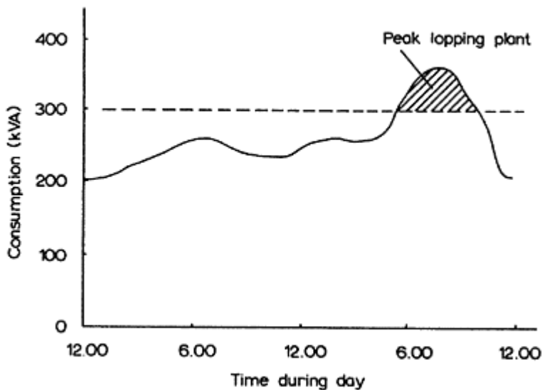
Figure 15.3 Load diagram
