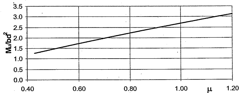
E-Effect of reinforcement ratio \mu
