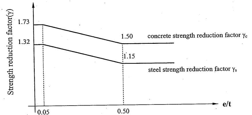
Fig. 1.11 Concrete and steel strength reduction factors
