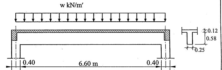
Fig. Ex-6.5a Simple beam
