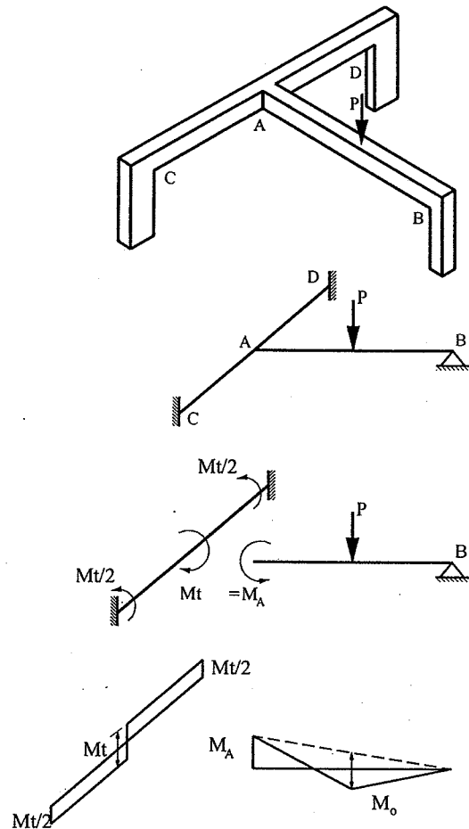
Fig. 8.2 Compatibility torsion
