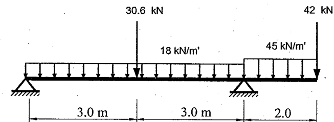
Load case 2
