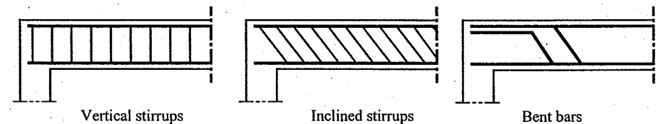
Fig. 4.9 Web reinforcements of reinforced concrete beams
