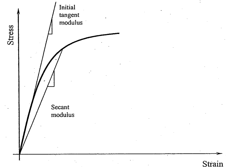
Fig. 1.8 Initial tangent modulus of concrete
