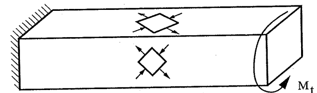
b) Principal stresses
