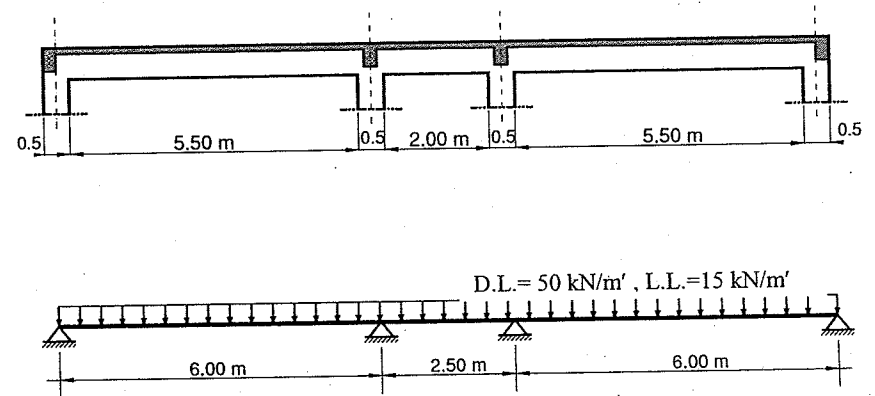
Fig. EX. 6.9a
