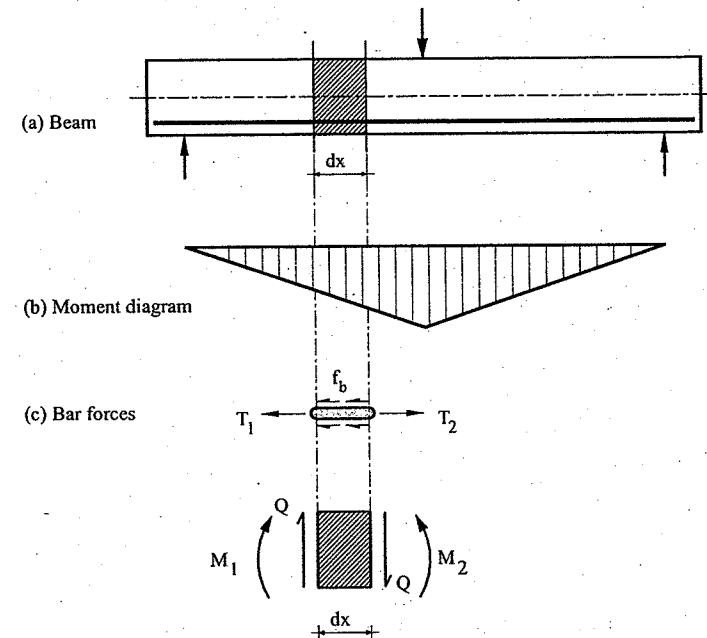
Fig. 5.2 Average flexural bond stress
