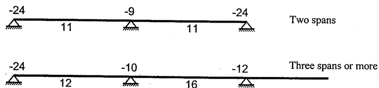
Fig. 6.10a Moment coefficients ( k_m ) for continuous beams
