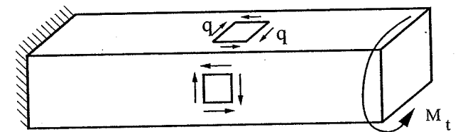
a) Shear stresses due to torsion
