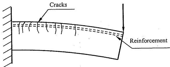
B-Cantilever beam
