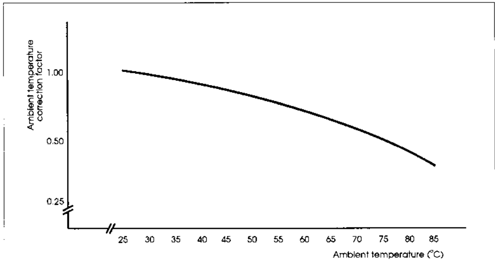
Figure 10.13: Typical temperature correction curve
