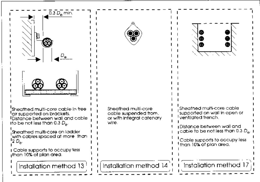
Figure 10.10: Reference method 13
