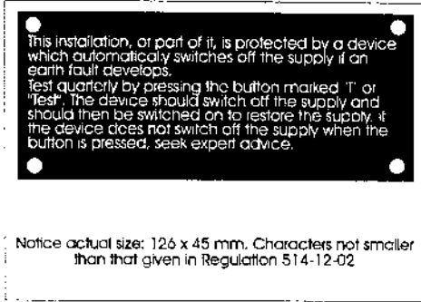
Figure 9.2: RCD notice
