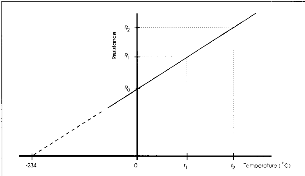
Figure 5.3: Variation of resistance of copper with temperature
