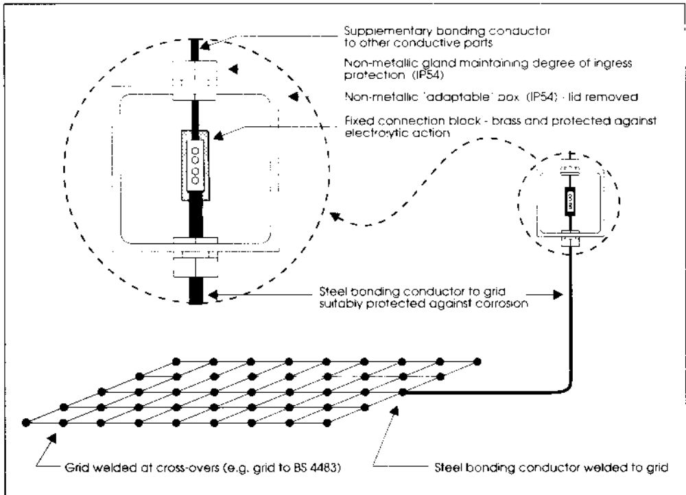
Figure 16.3: Typical method of connection of equipotentially bonded grid in Zones B and C
