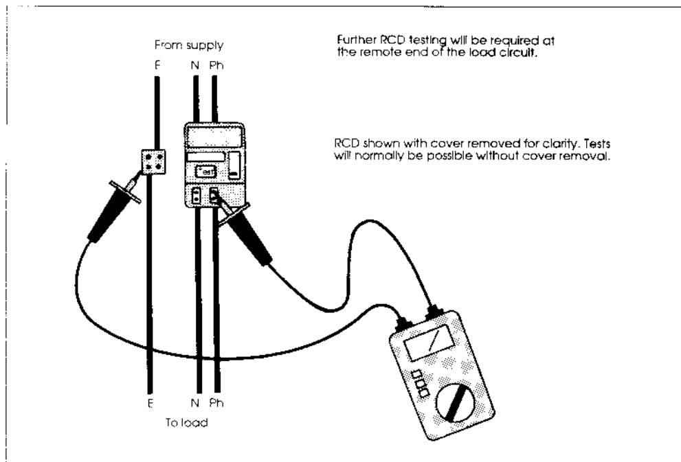
Figure 17.10: RCD testing
