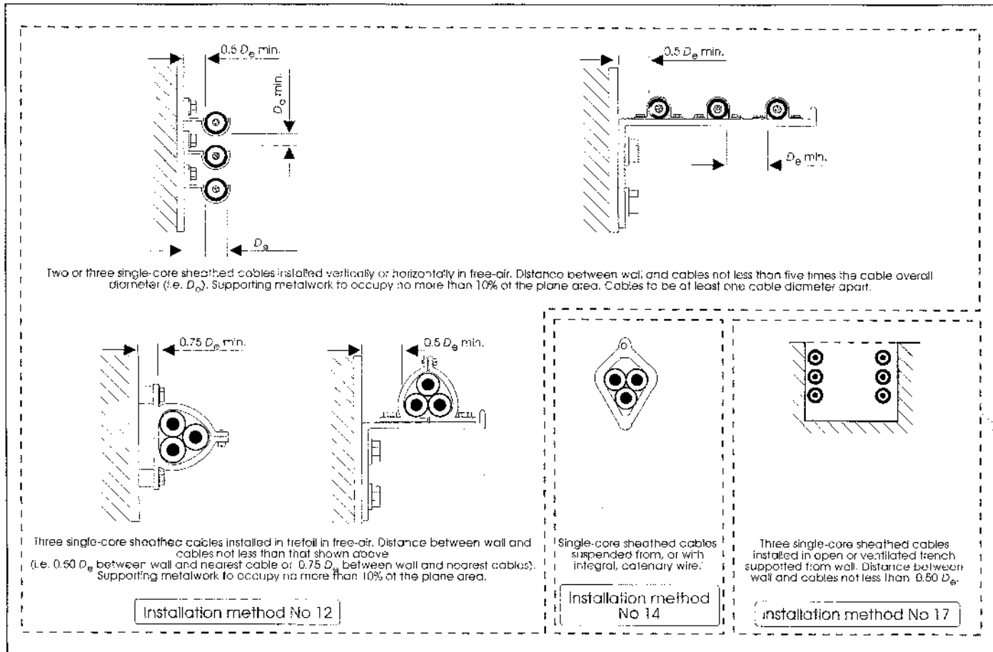
Figure 10.8: Reference method 12
