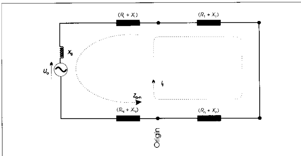
Figure 7.6: Phase-to-neutral fault equivalent circuit
