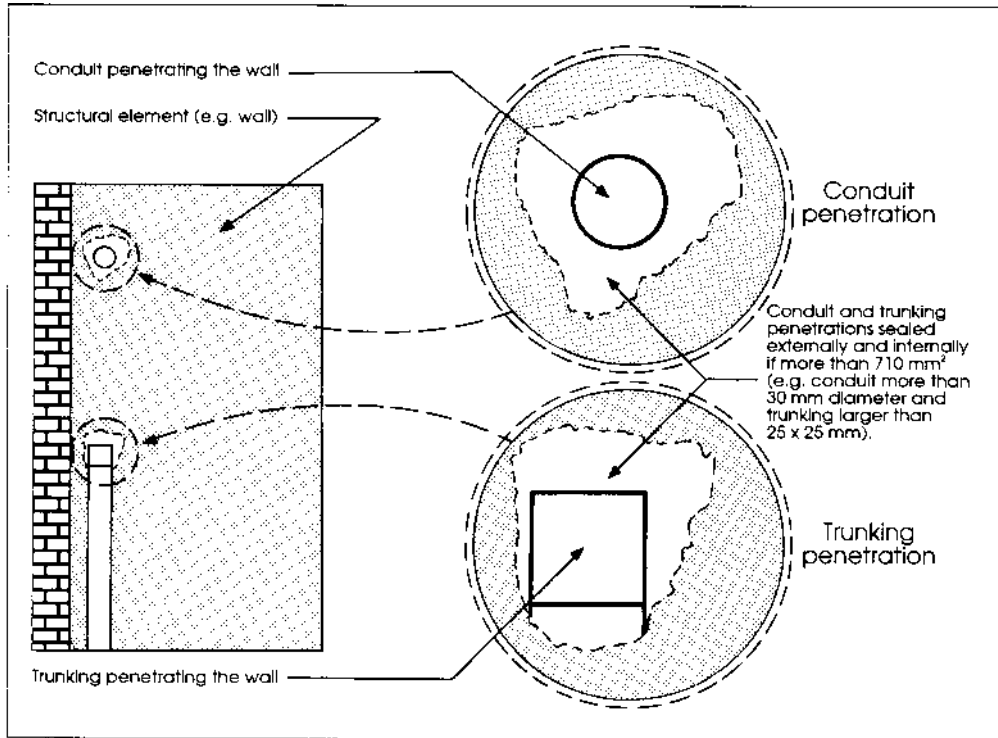
Figure 10.17: Sealing of wiring system penetrations
