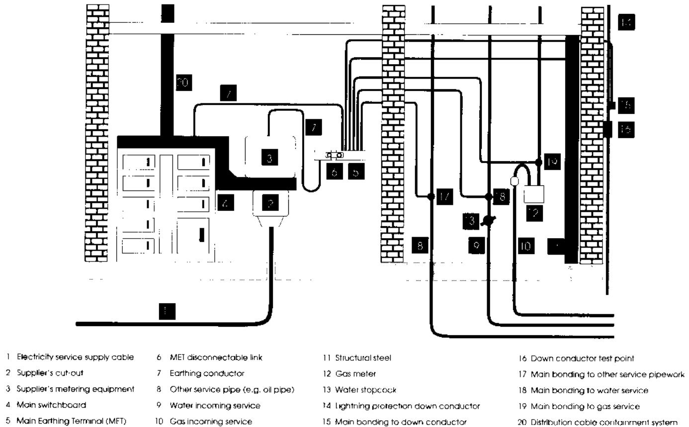
Figure 12.9: Typical main bonding connections
