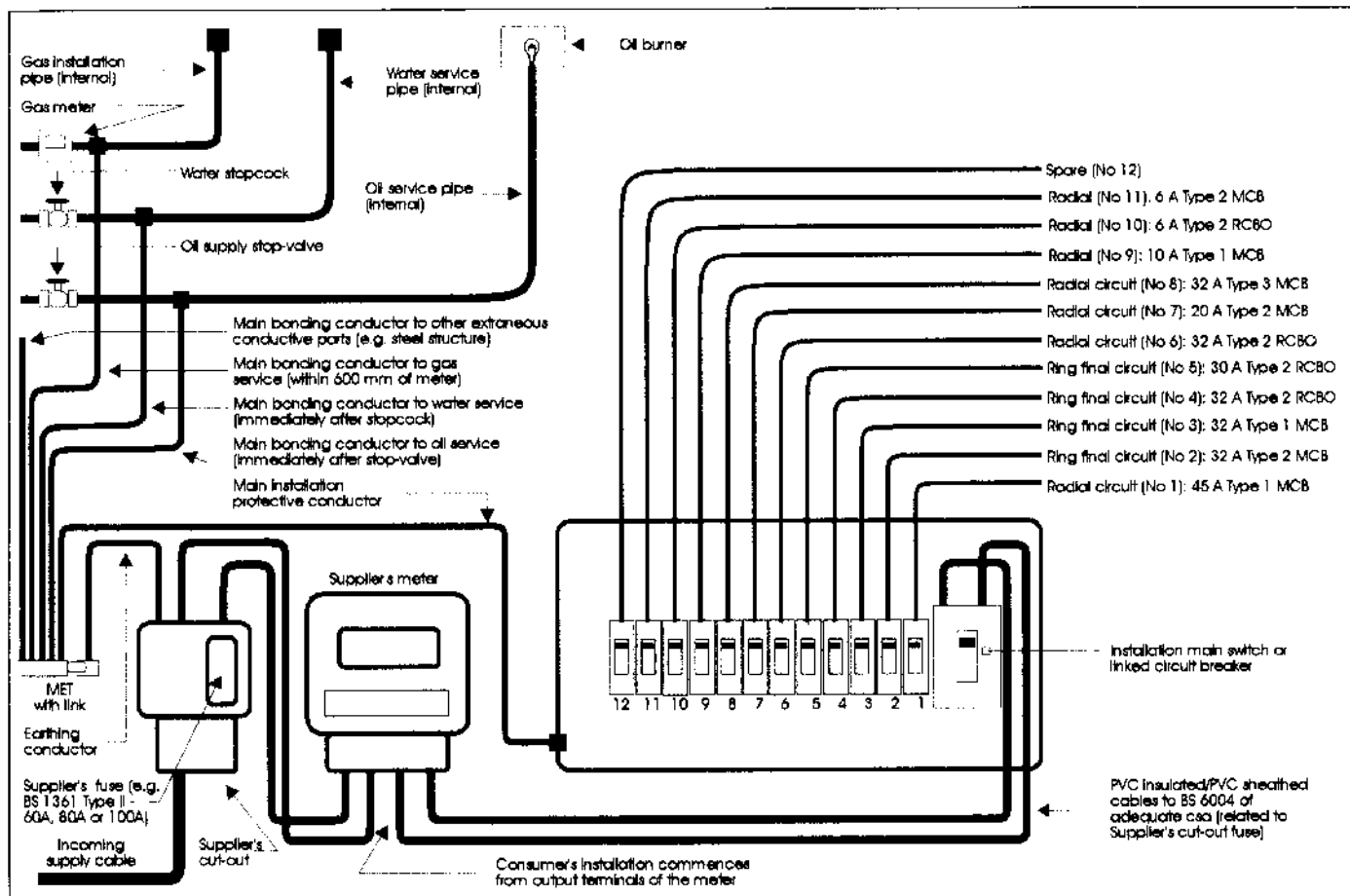
Figure 15.5: Typical small installation layout – TN-S system
