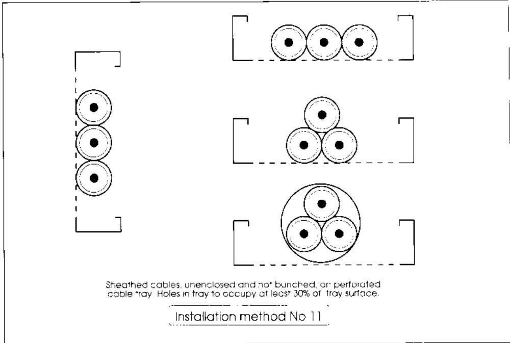
Figure 10.9: Reference method 11
