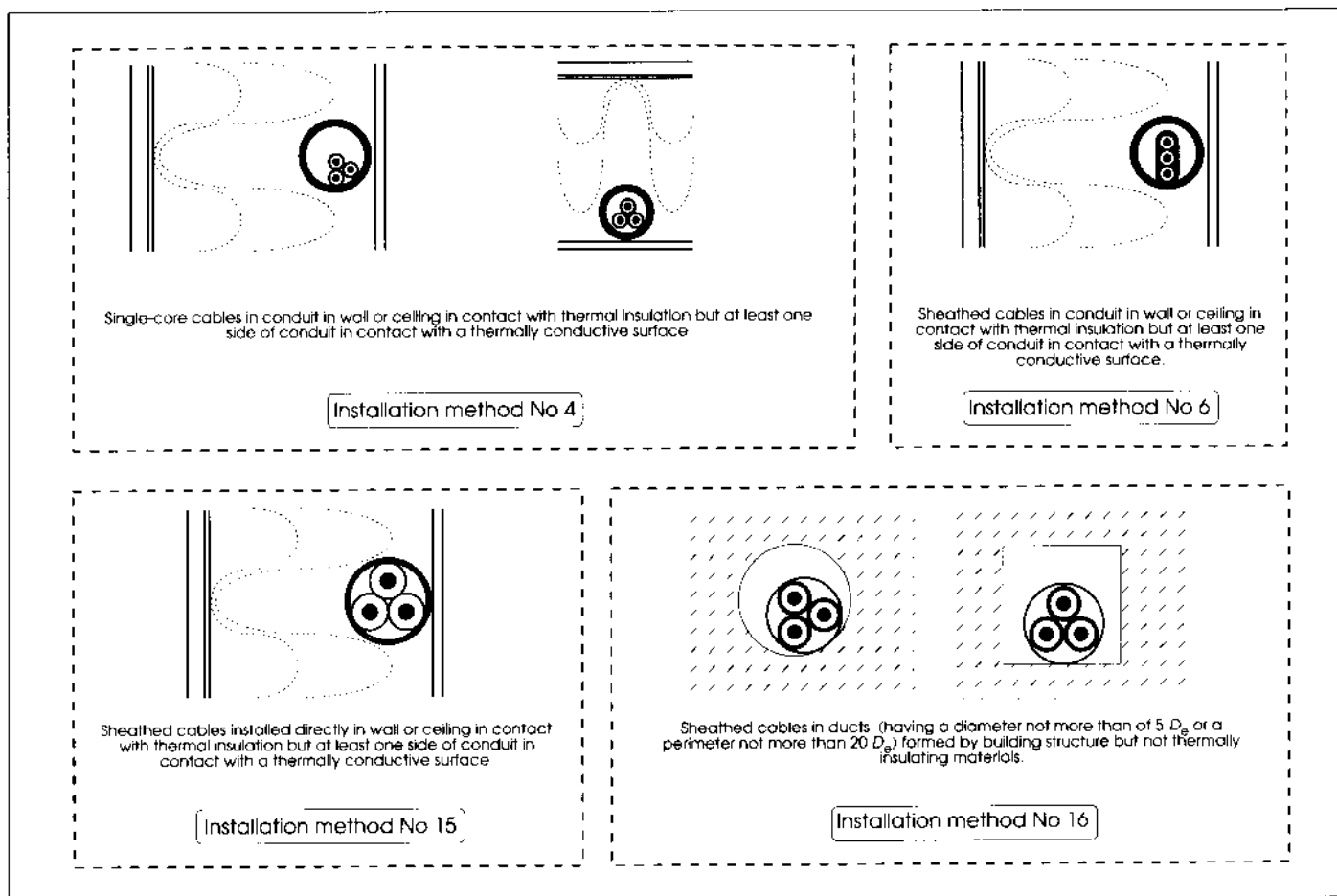
Figure 10.7: Reference method 4
