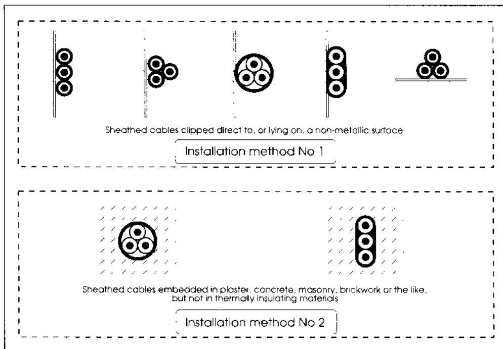
Figure 10.5: Reference method 1
