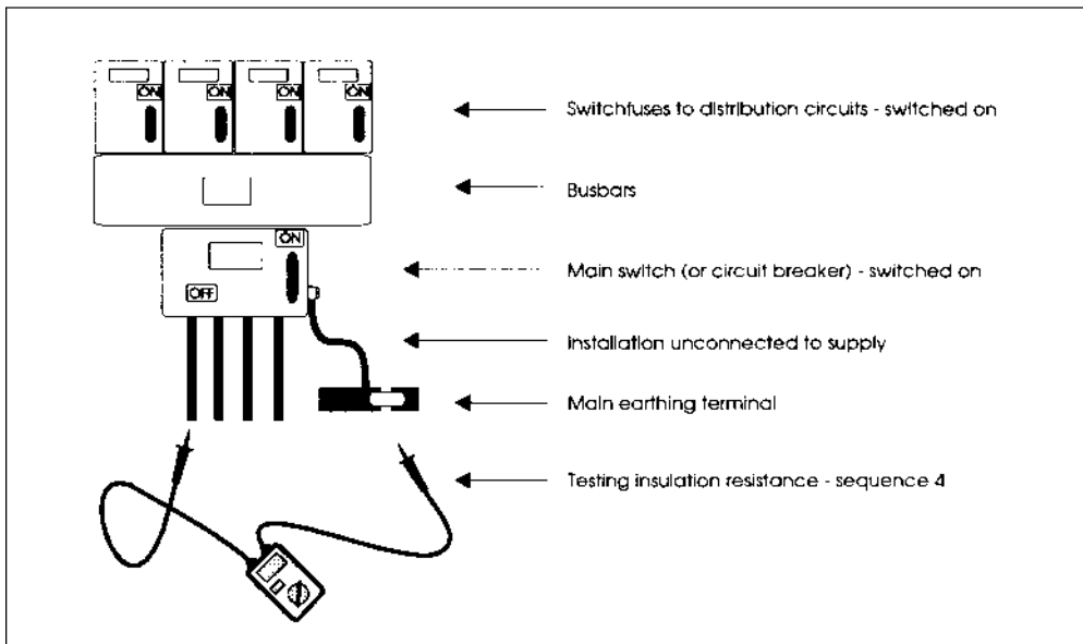
Figure 17.3: Testing insulation
