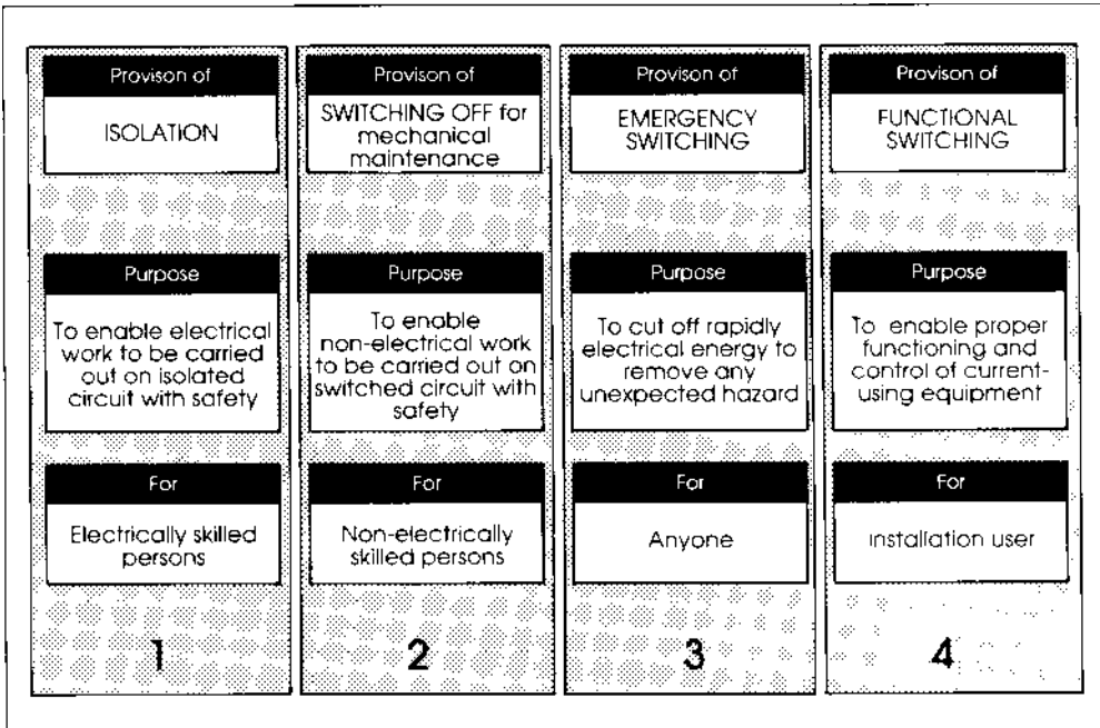
Figure 8.1: Isolation and switching – the four concepts
