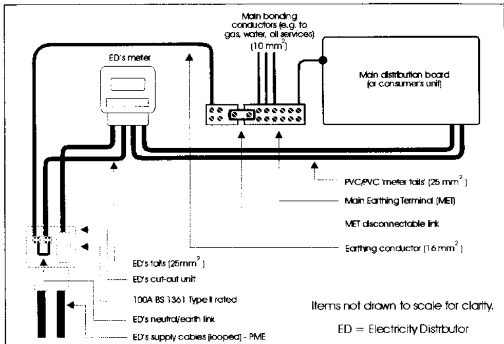
Figure 15.1: Typical arrangement for connection of a smaller installation on a TN-C-S system
