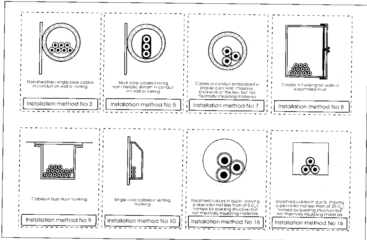
Figure 10.6: Reference method 3
