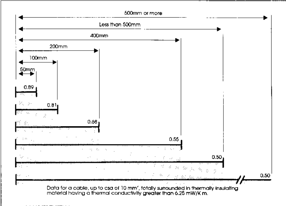
Figure 10.14: Derating of a cable when installed in thermally insulating material
