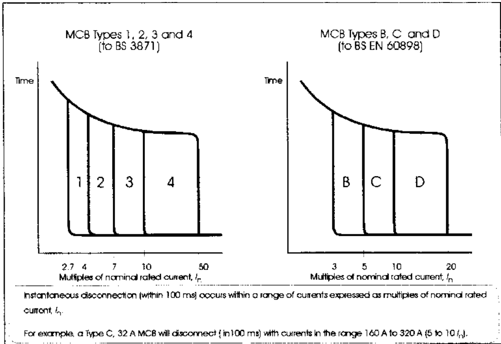
Figure 11.9: MCB characteristics
