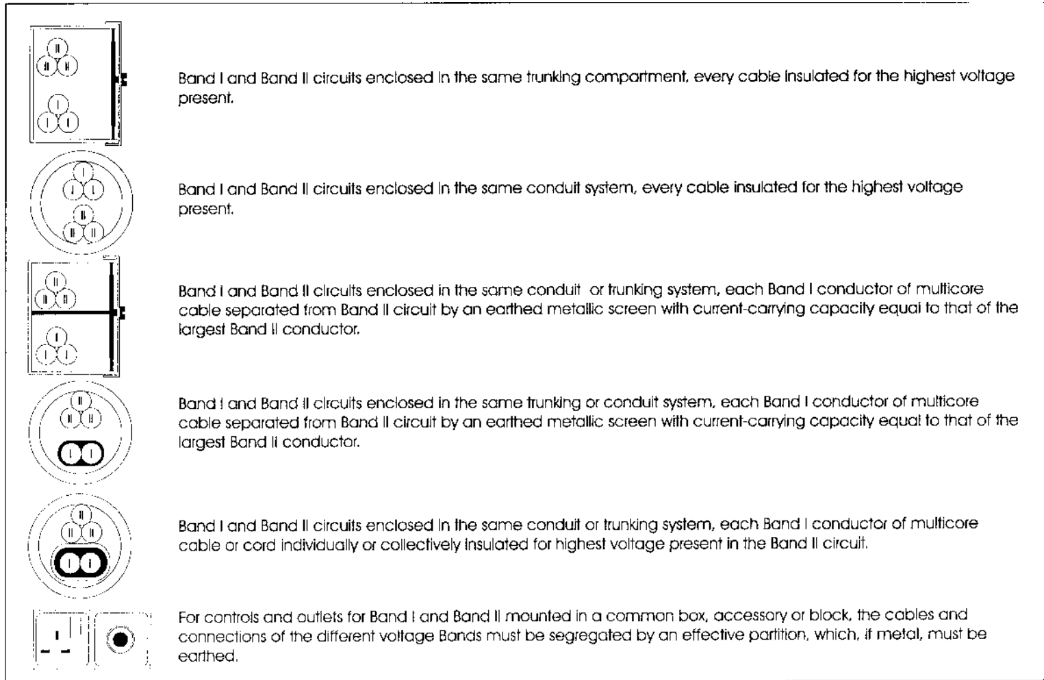
Figure 10.4: Examples of circuit segregation (Band I and Band II circuits)
