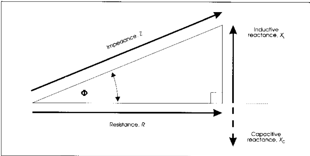
Figure 7.5: Impedance triangle
