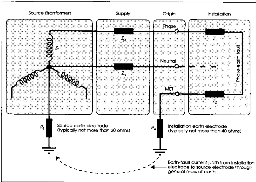
Figure 11.19: TT system circuit under earth fault conditions
