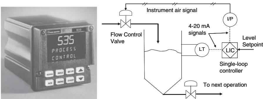
Figure 17.19 A typical process controller and a schematic diagram of the liquid level control system.
