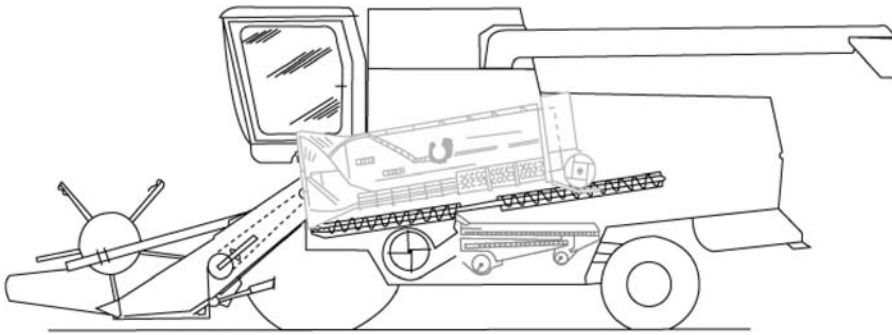
Figure 5.7 Rotary-type of combine threshing.
