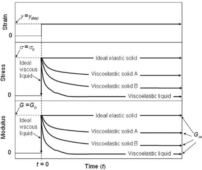
Figure 14.16 Responses of different materials during stress relaxation tests.
