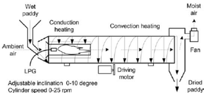
Figure 9.1 A Schematic drawing of combined conduction and convection type rotary dryer (Courtesy: Likitattanaporn et al. , 2003).
