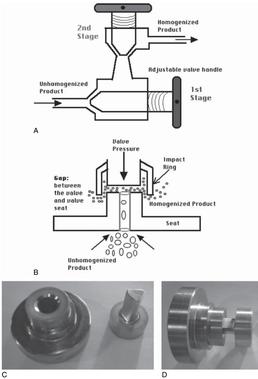
Figure 8.6 Homogenizing valve for dairy products. A) Flow of product through the valve assembly, showing incoming unhomogenized product from the pump passing through the first and second stages before exiting. B) Schematic diagram of the homogenizing valve. C) and D) Pictures of homogenizing valve depicted in B.
