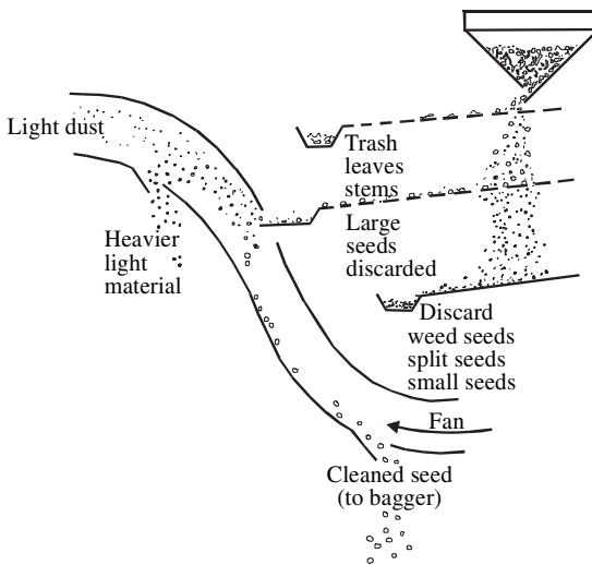
Figure 6.12 Fanning mill.
