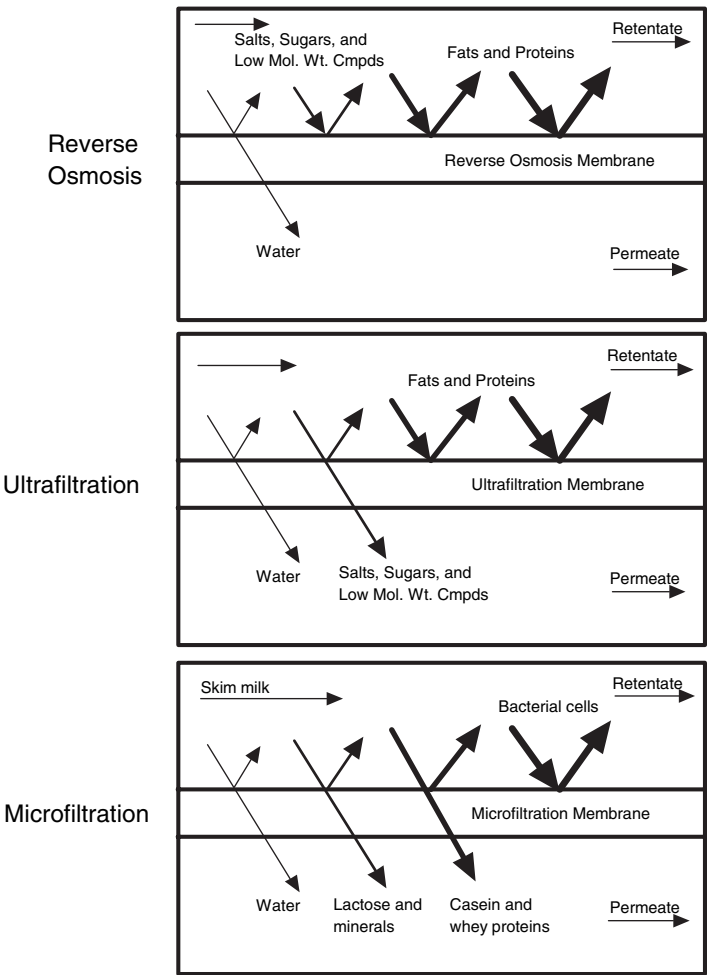
Figure 8.7 Passage of components through different types of membranes used in milk and dairy product processing.
