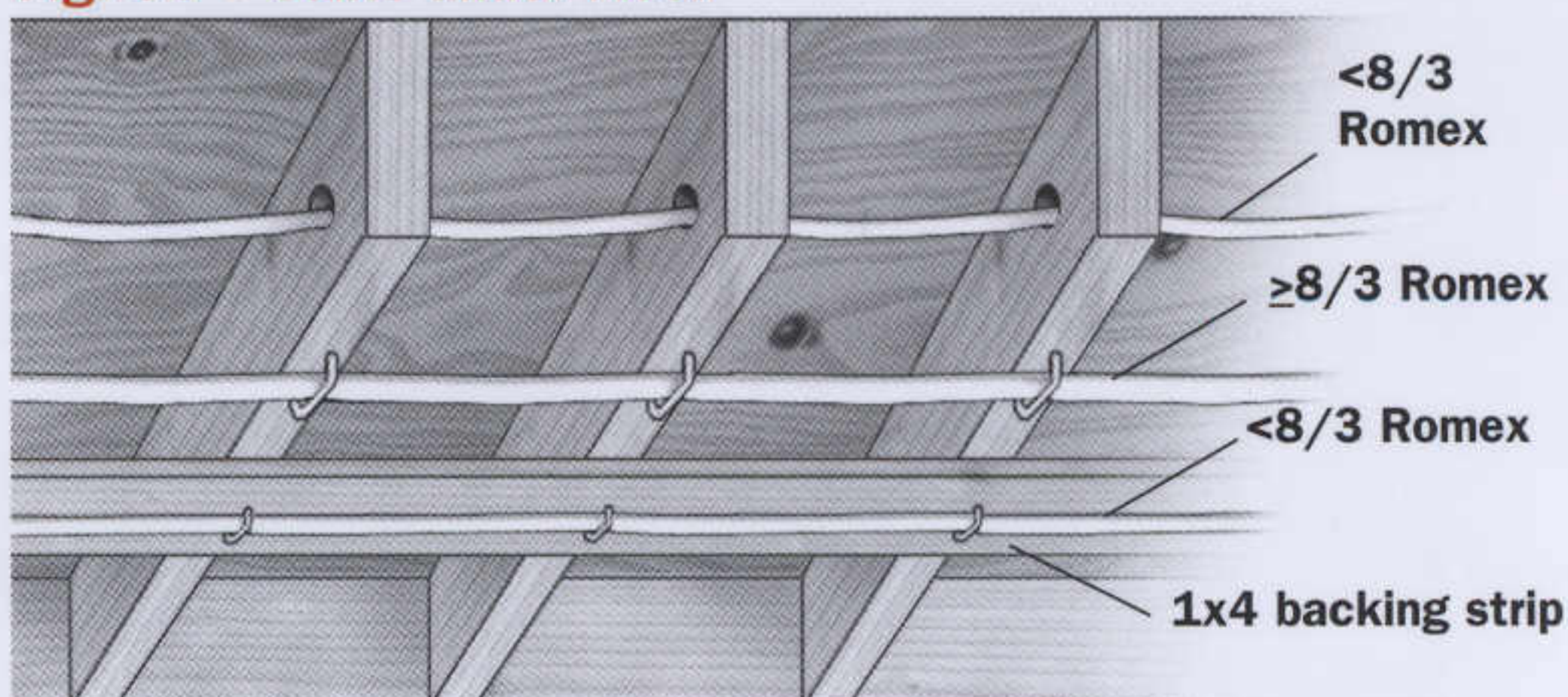
Fig. 54 • Cable under Floor
