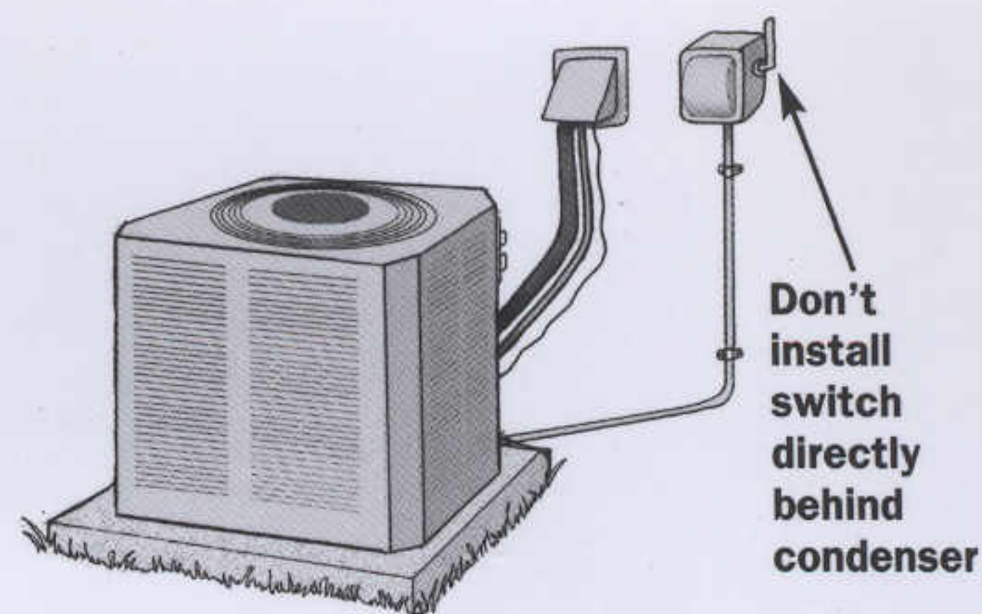
Fig. 73 Air-Conditioning Condenser
