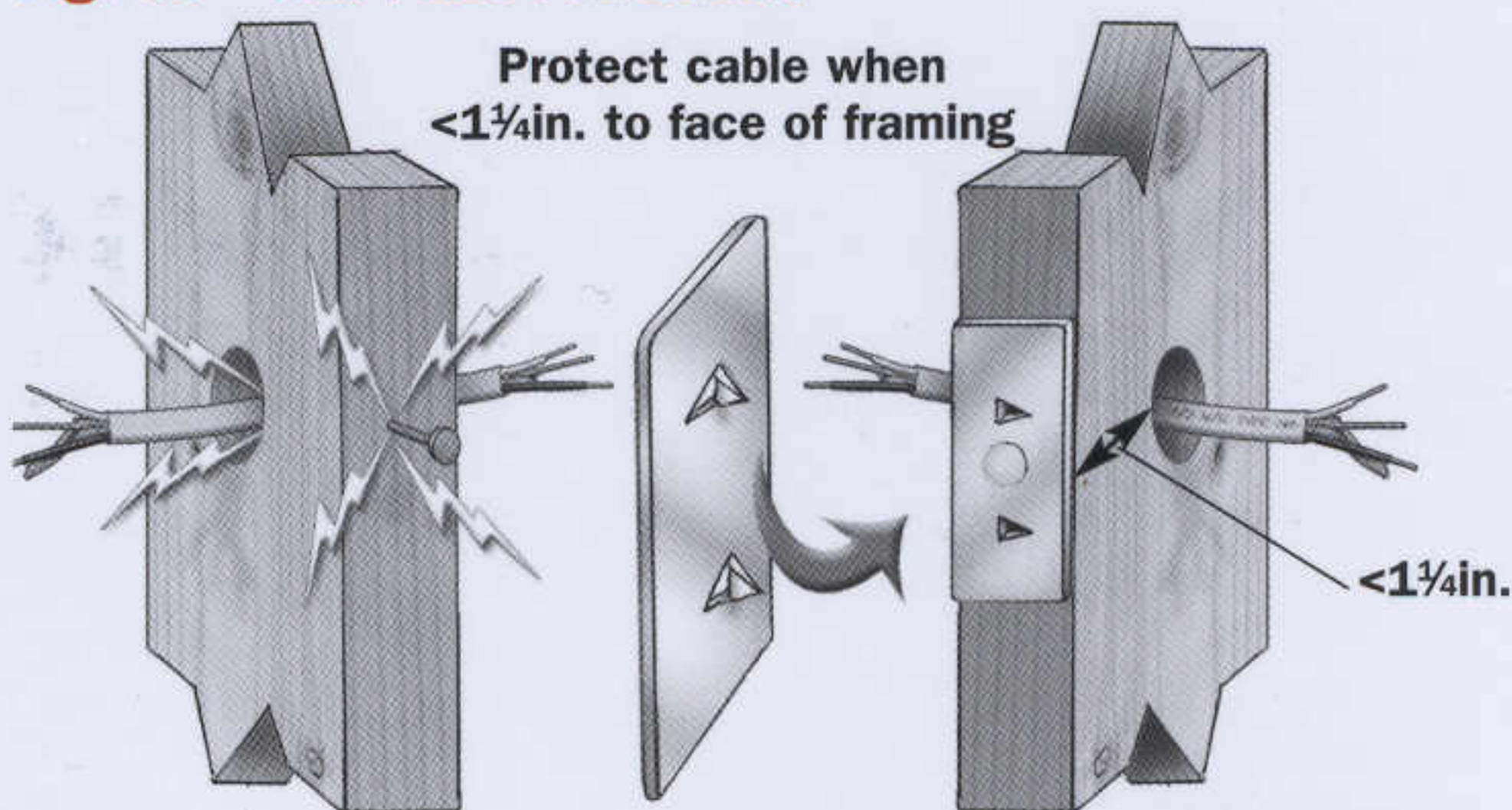
Fig. 55 • Nail-Plate Protection
