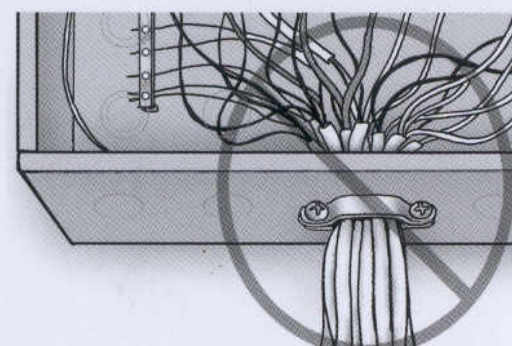
Fig. 33 Improper Cable Bundle
