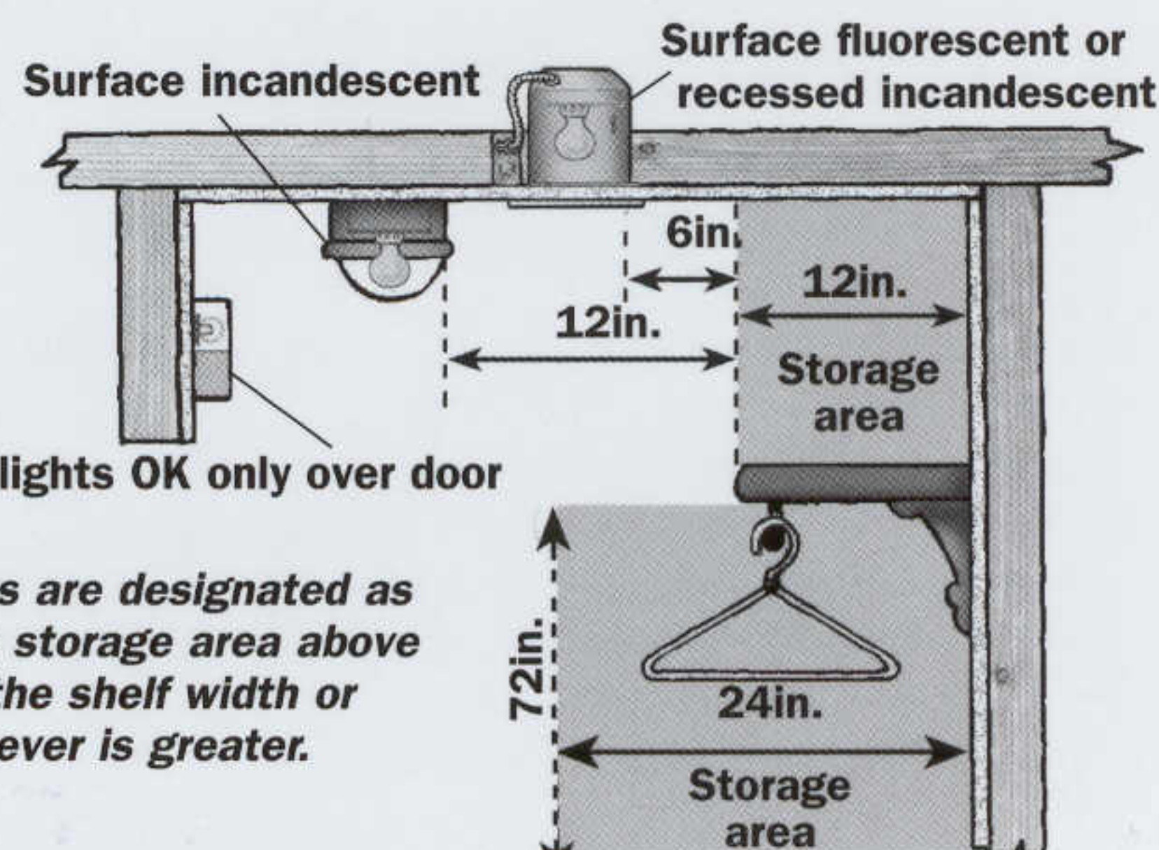
Fig. 78 Closet Lights
