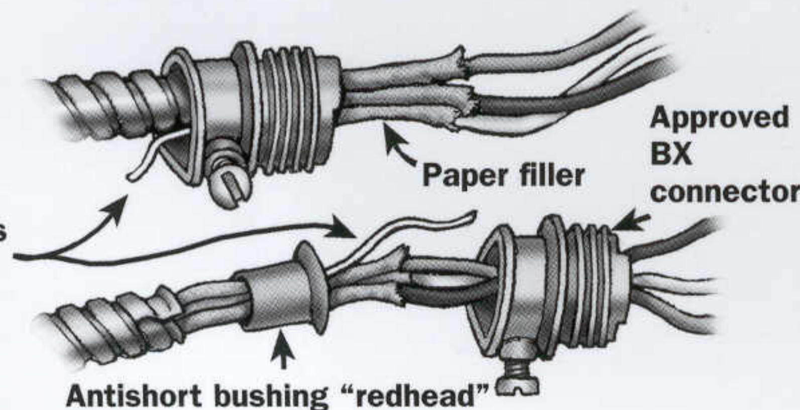
Fig. 46 BX—Armored Cable
