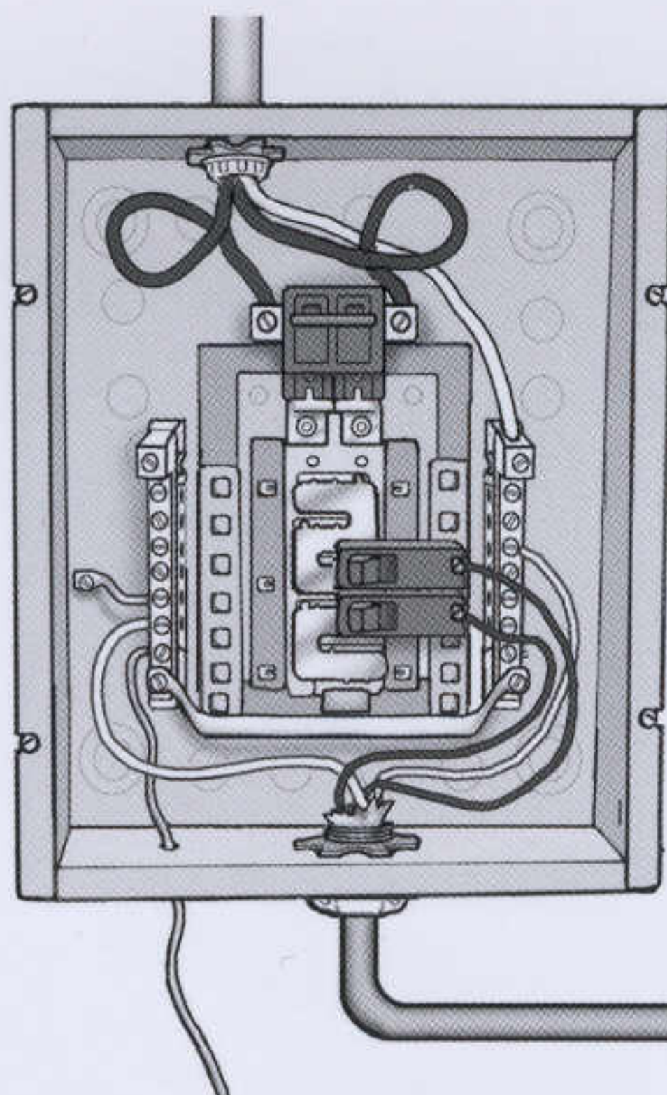
Fig. 31 Service Panel
