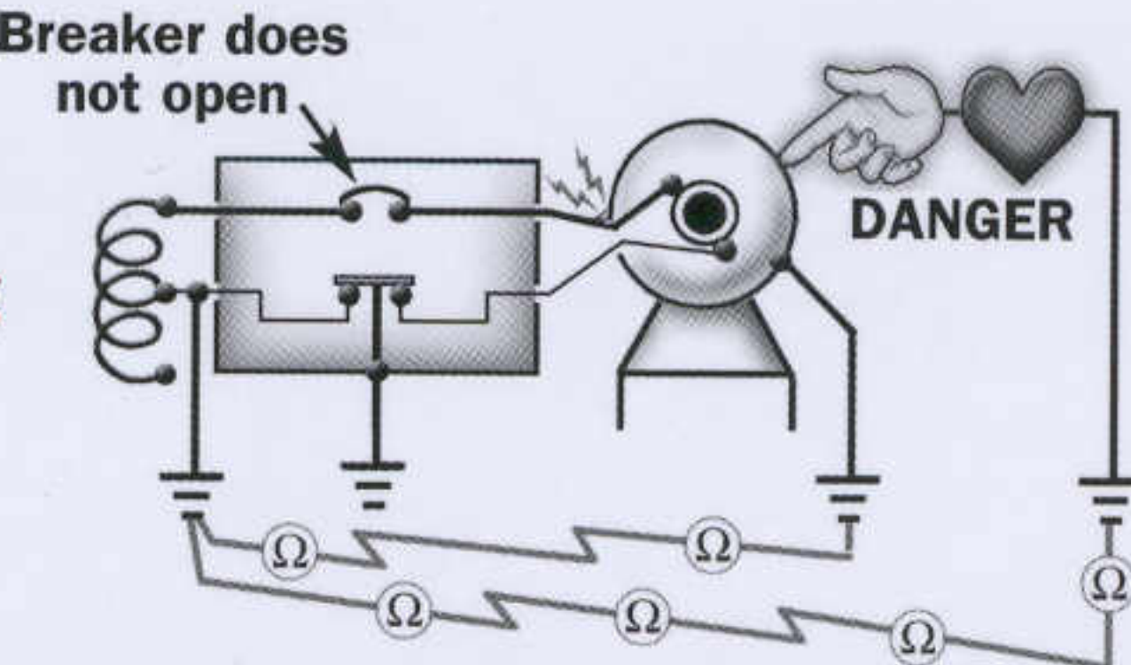
Fig. 15 Futility of Using Earth as the Equipment Ground
