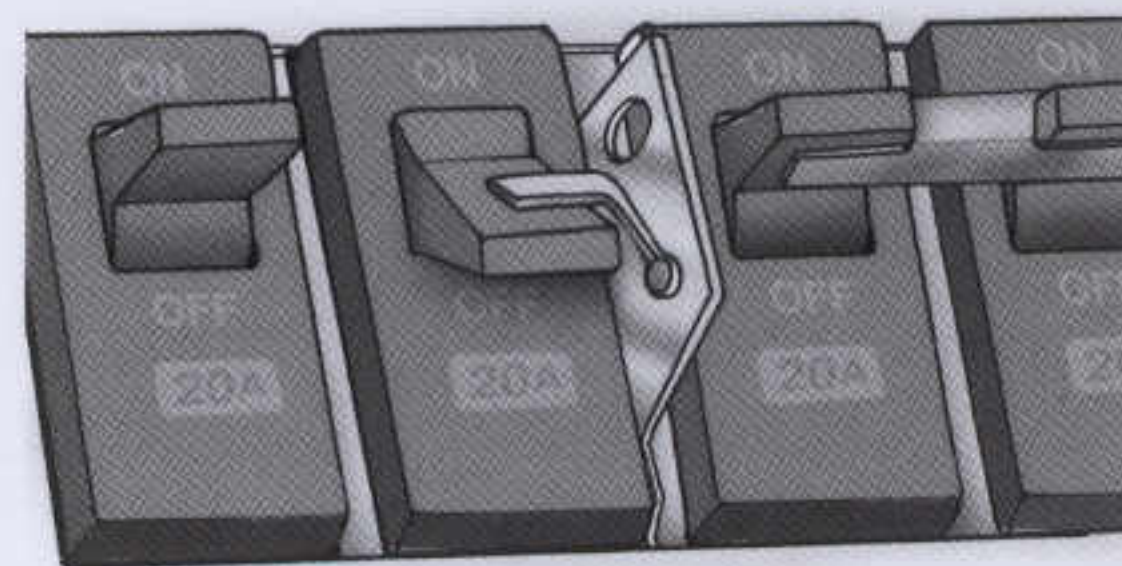
Fig. 74 Breaker Lockout
