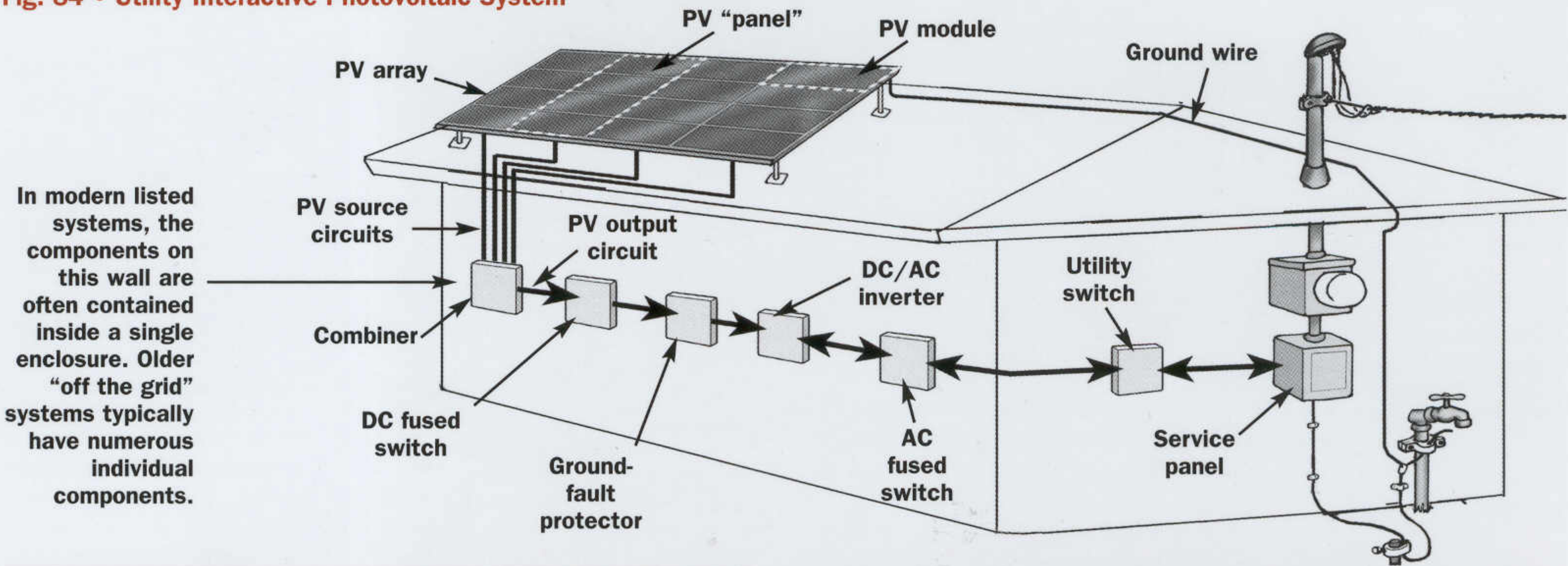
Fig. 84 • Utility Interactive Photovoltaic System
