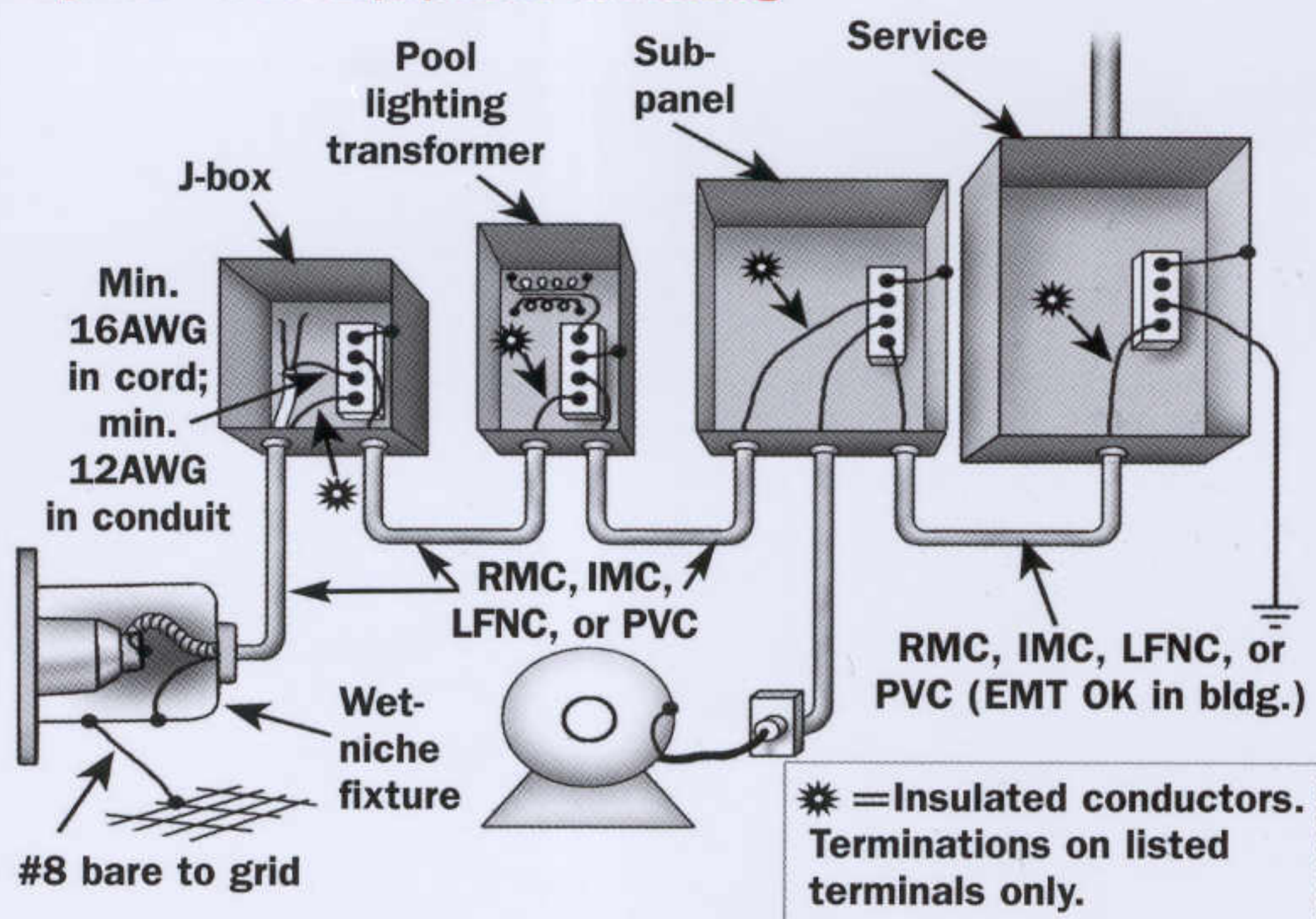
Fig. 81 • Pool Equipment Grounding
