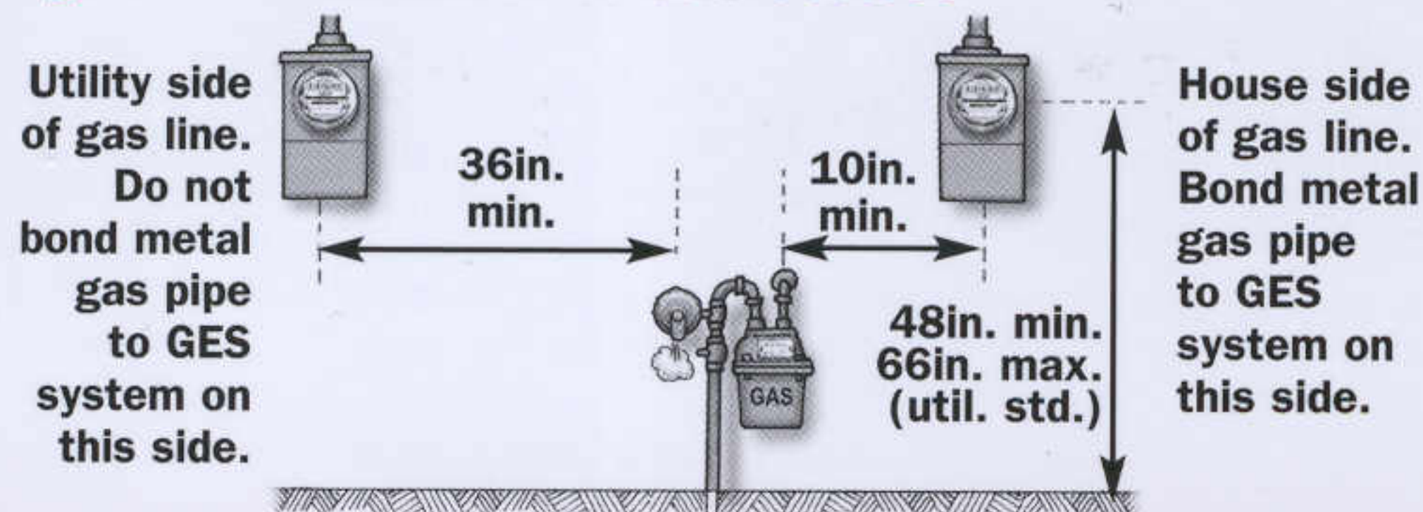
Fig. 25 • Clearances to Gas Service
