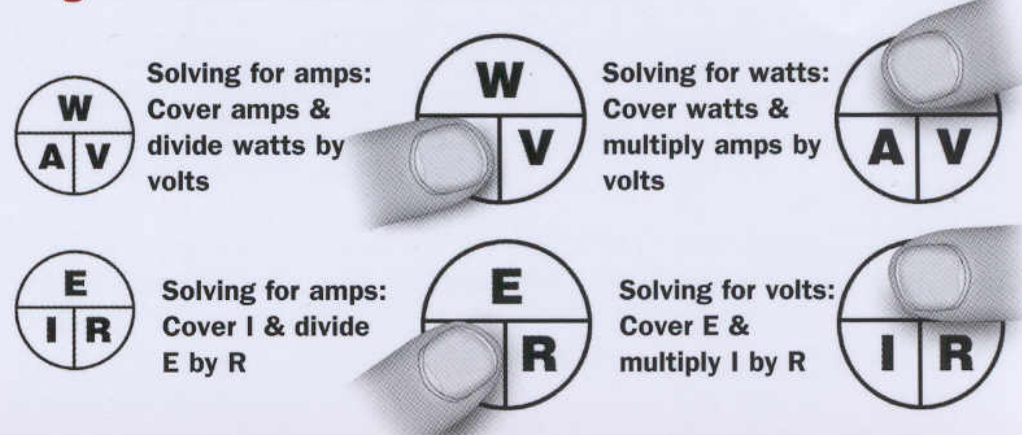
Fig. 3 • Ohm's Law & Power Formula
