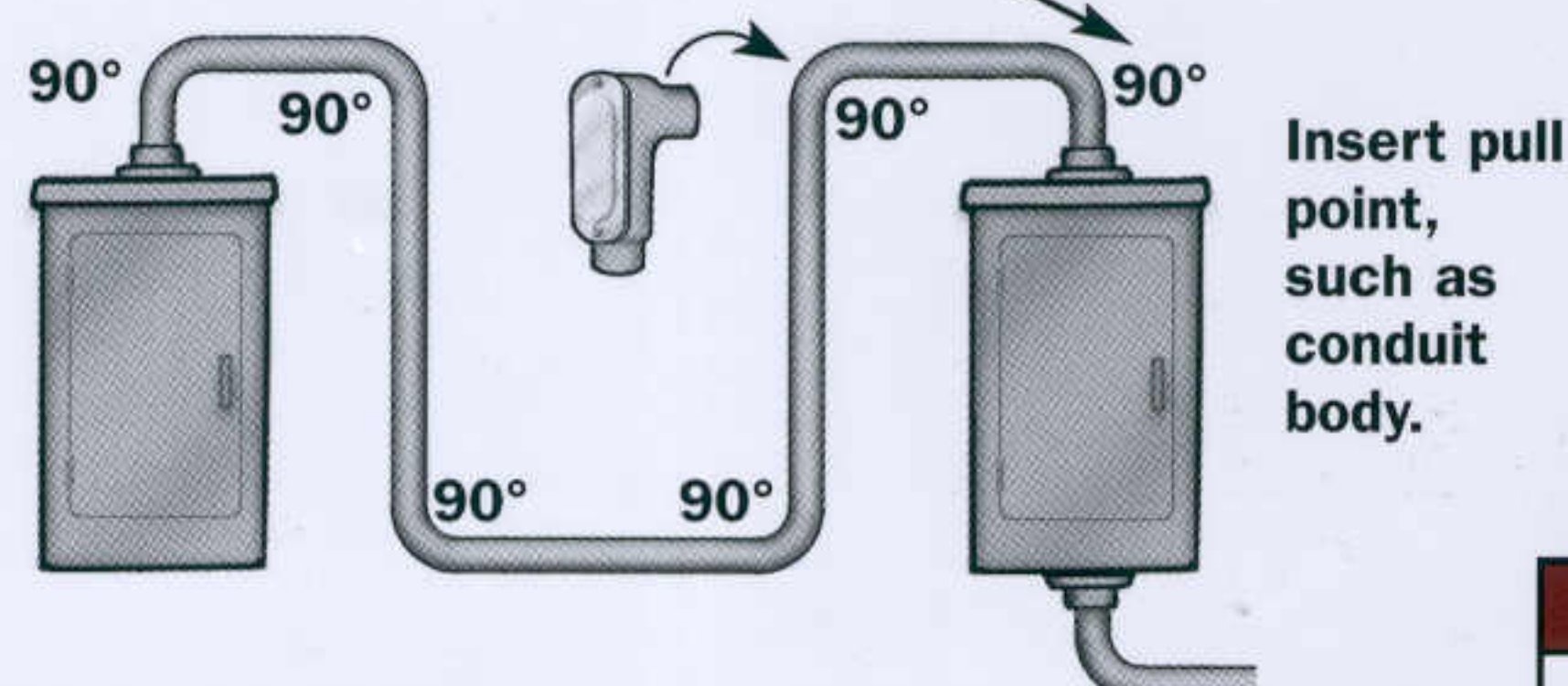
Fig. 63 • Too Many Bends 6 x 90° = 540° = violation
