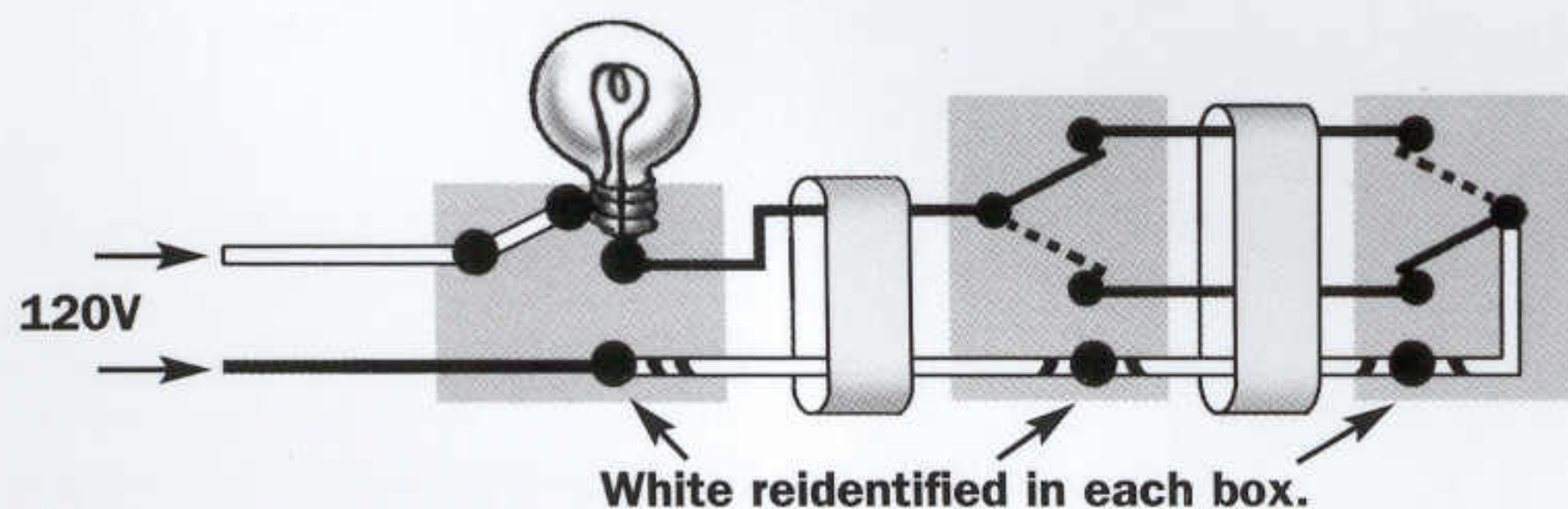
Fig. 80 • 4-Way Switch
