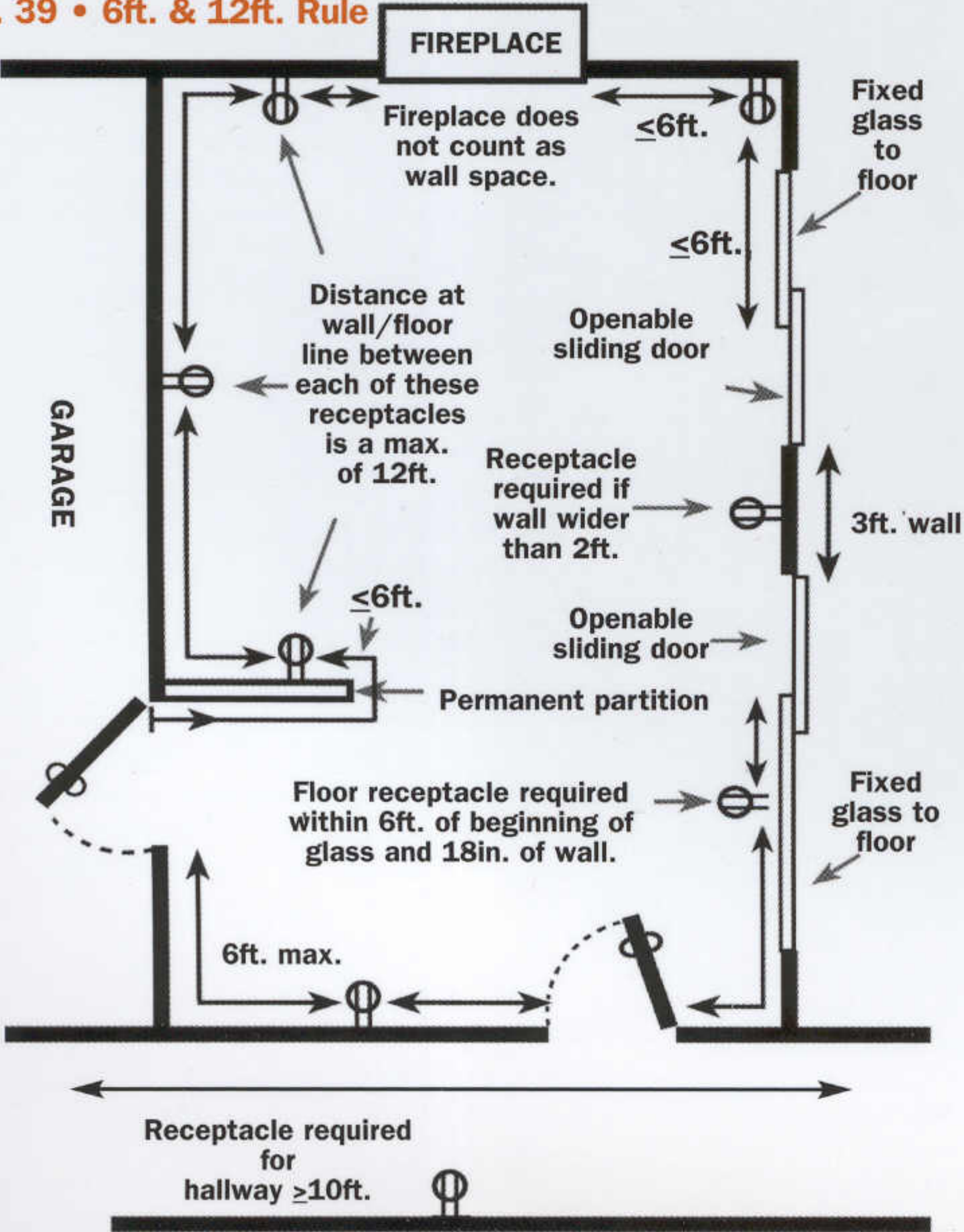
Fig. 39 • 6ft. & 12ft. Rule
