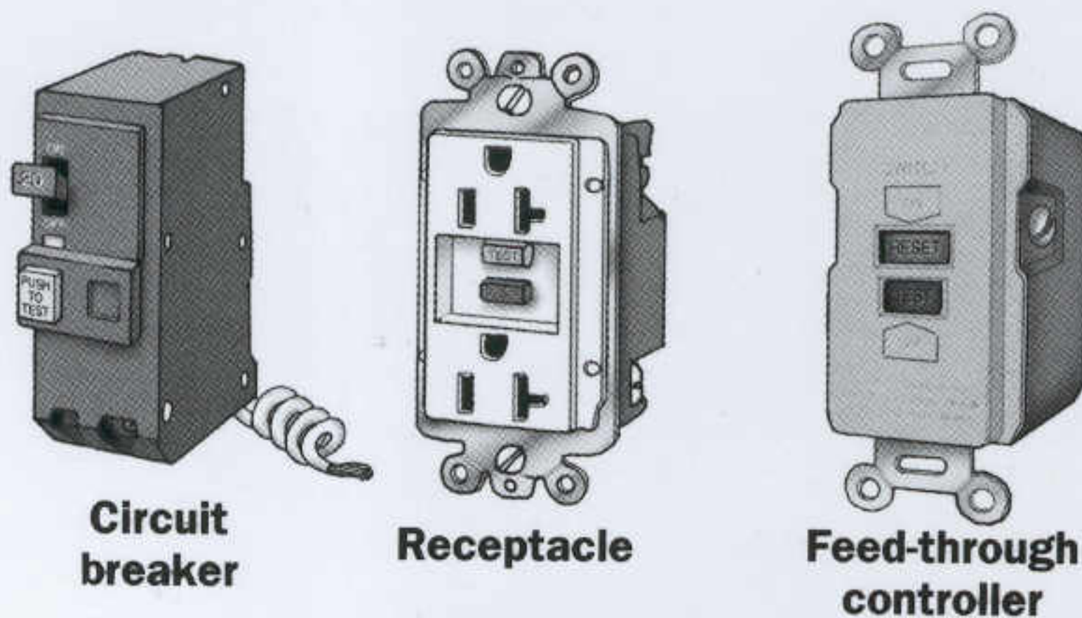
Fig. 17 • Three GFCIs
