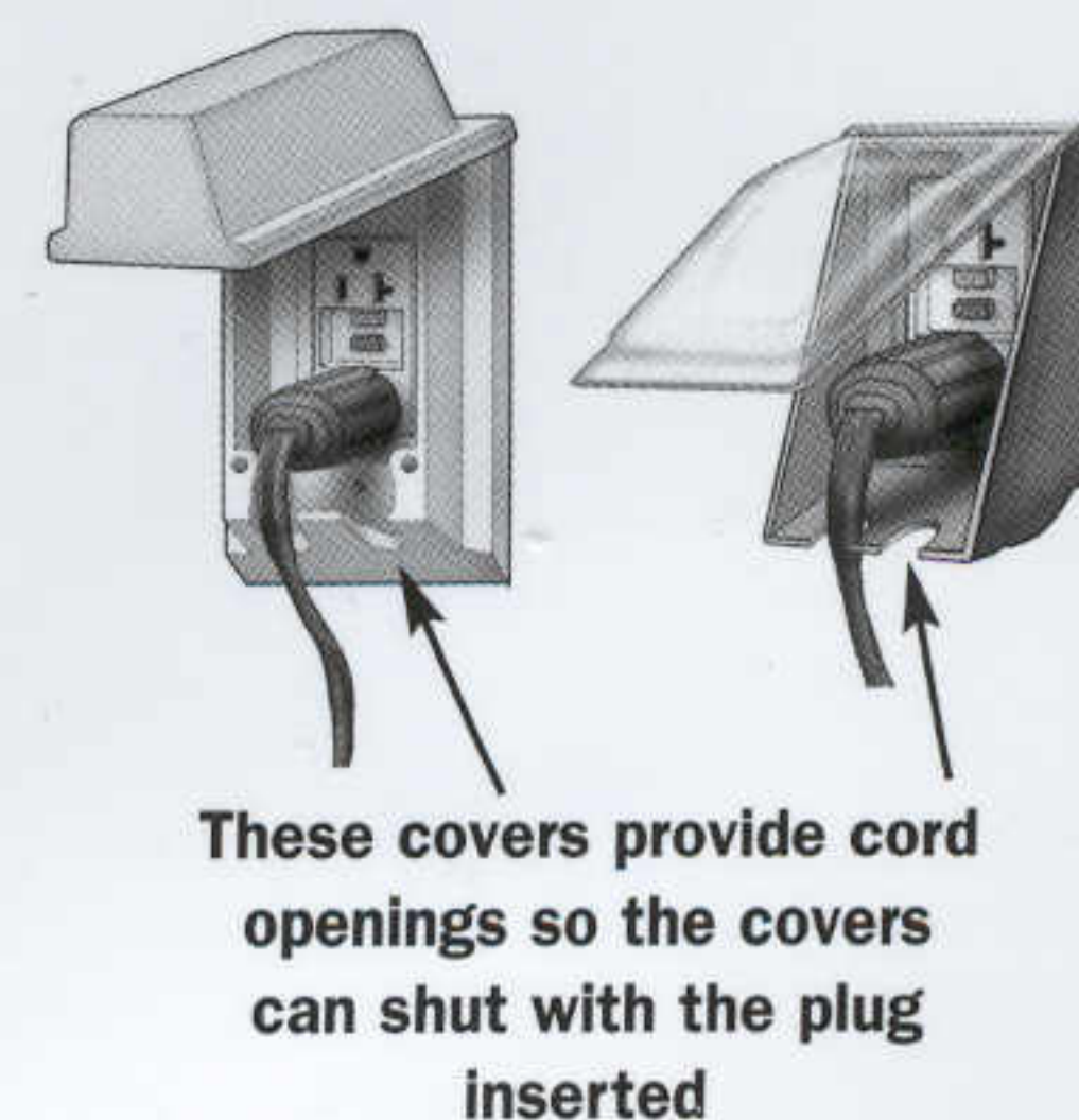
Fig. 70 In-Use Covers
