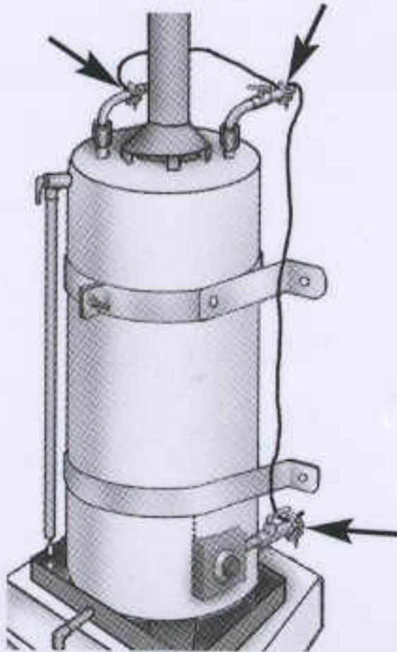
Fig. 12 • Bonding the Piping System
