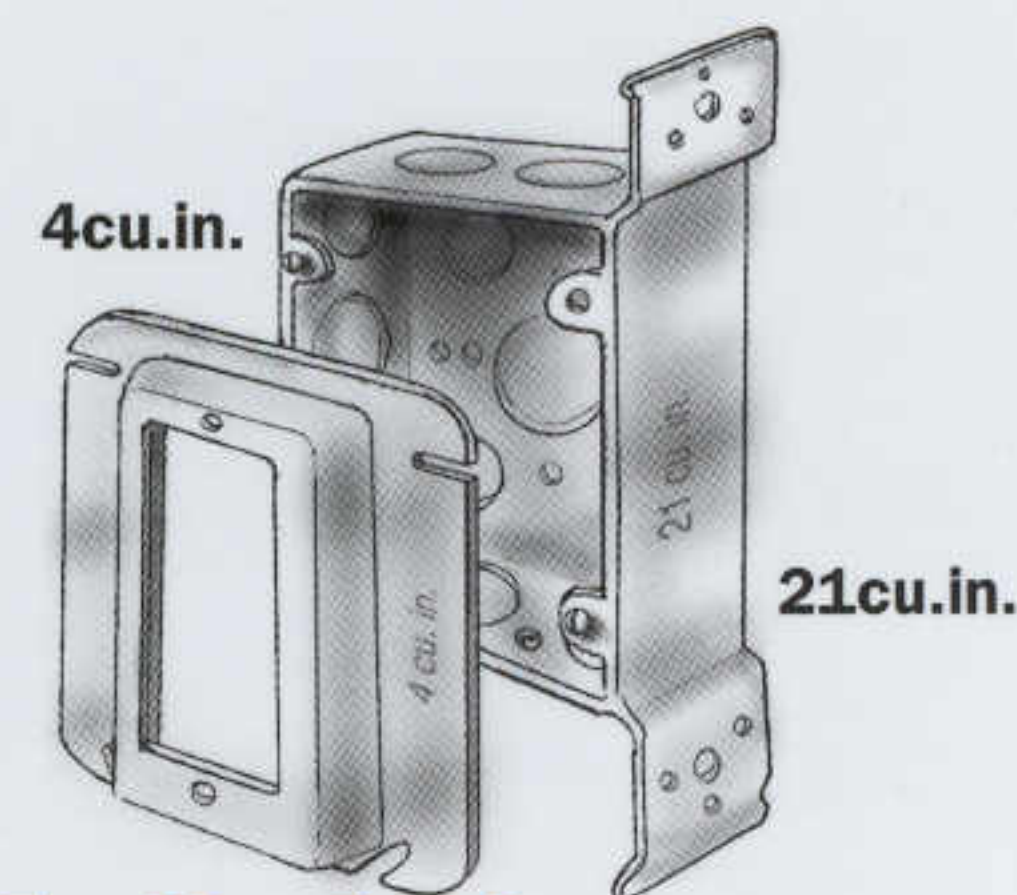
Fig. 68 • Four-Square Steel/Side Bracket
