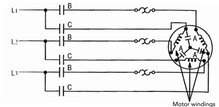
Figure 4.5 Wye-Delta Starter
