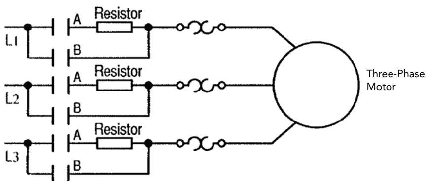
Figure 4.3 Primary Resistance Starter
