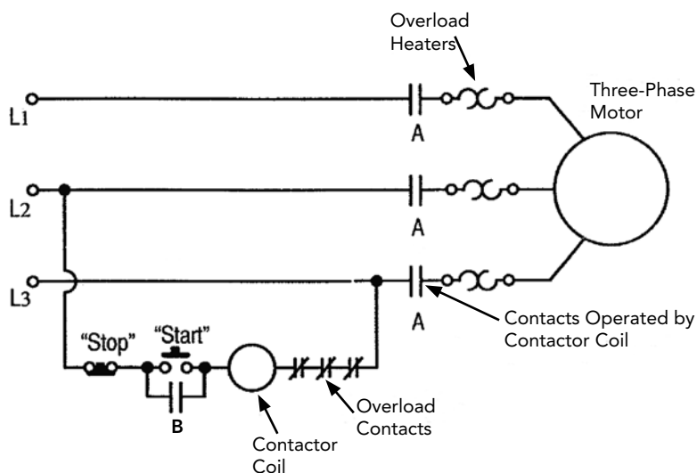
Figure 4.2 Magnetic Starter
